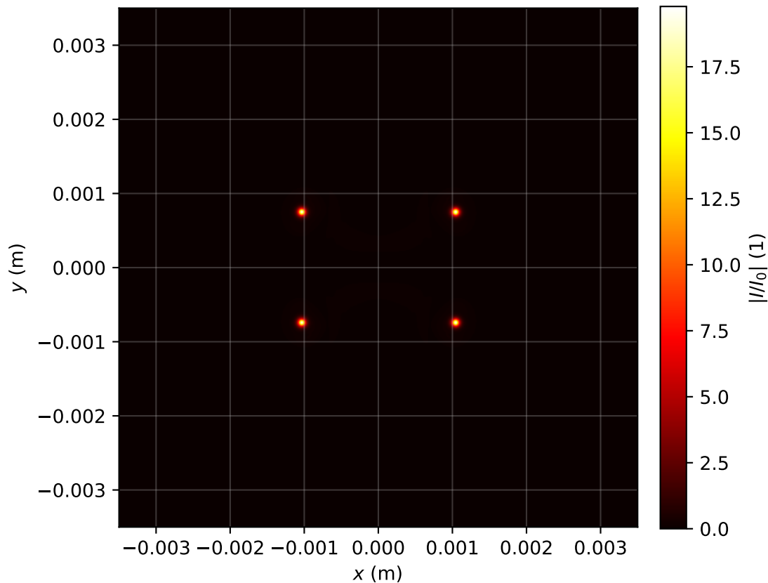
Intensity profile I(x, y, z = 2.388)/I_0 , P_{in}=8.0P_{cr} , artificial time
